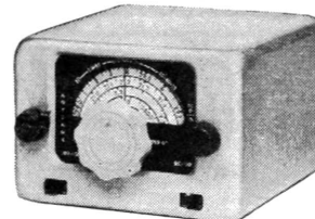
ECCO 10 METER TRANS-RECEIVER Designed for spot frequency use for emergency, CD, and net operation. Completely self-contained including batteries. Transmitter uses 20 meter crystals. Fixed frequency receiver has regenerative circuit. Base loaded 36" antenna. Carbon mike input. 1/2 watt input to final. With 5 tubes. Less mike, headphones, crystal, and batteries. MODEL HT-2. Net $74.50. Z-3 Crystal (specify frequency). Net $3.87. Batteries (2-M30 "B", 1-2F "A"). Net $4.76.
